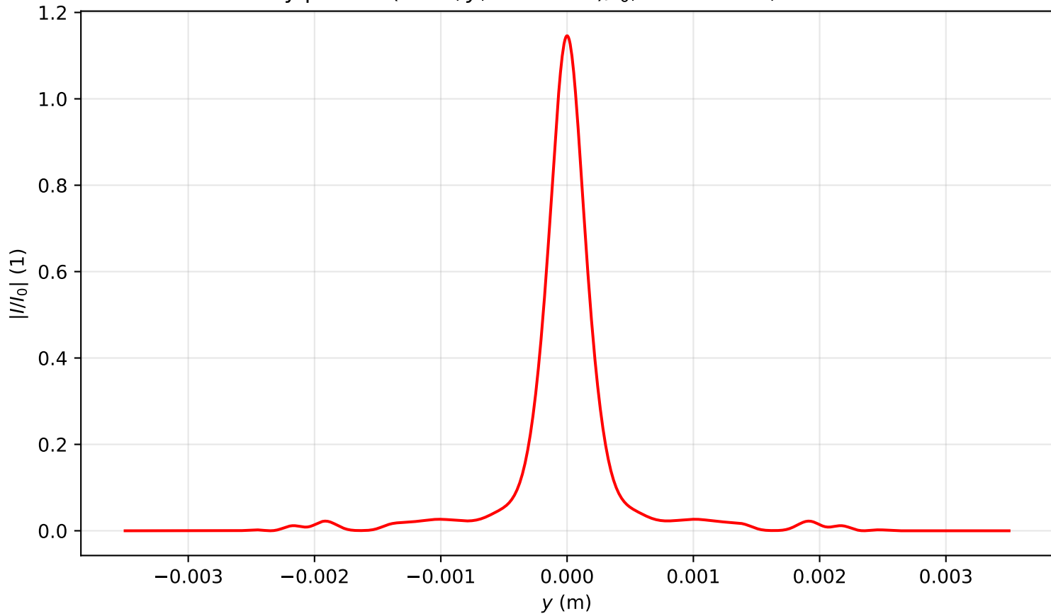
Intensity profile I(x=0, y, z=3.344)/I_0 , P_{in}=4.0P_{cr} , artificial time
